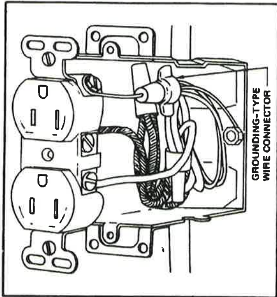
Fig. 5-21 An approved method of connecting the grounding conductor using a special grounding-type wire connector.
