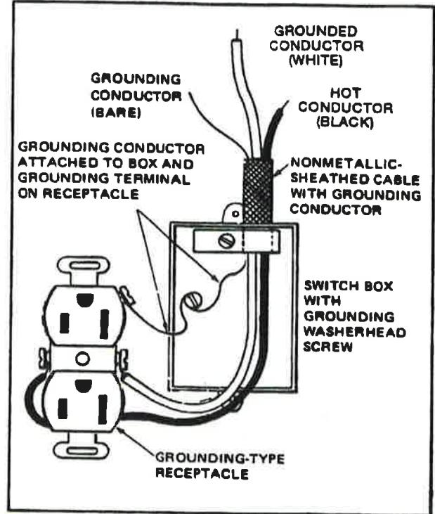
Fig. 5-20 Detail showing connections for grounding-type receptacles.
