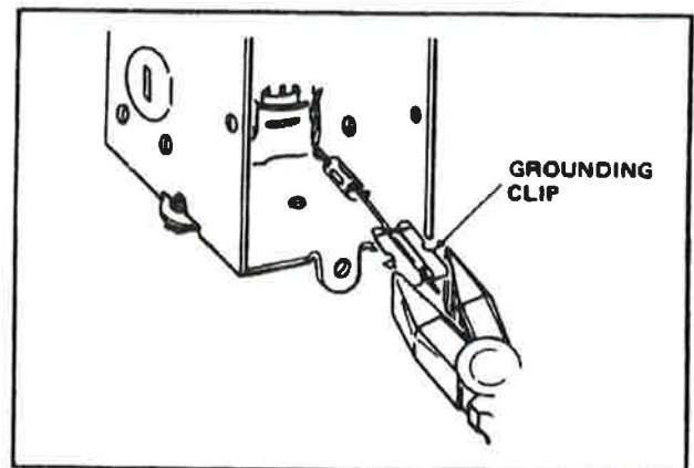
Fig. 5-22 Method of attaching grounding clip to switch (device) box.
