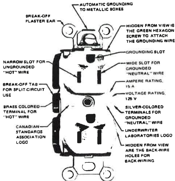
Fig. 5-23 Grounding-type receptacle detailing various parts of the receptacle.
